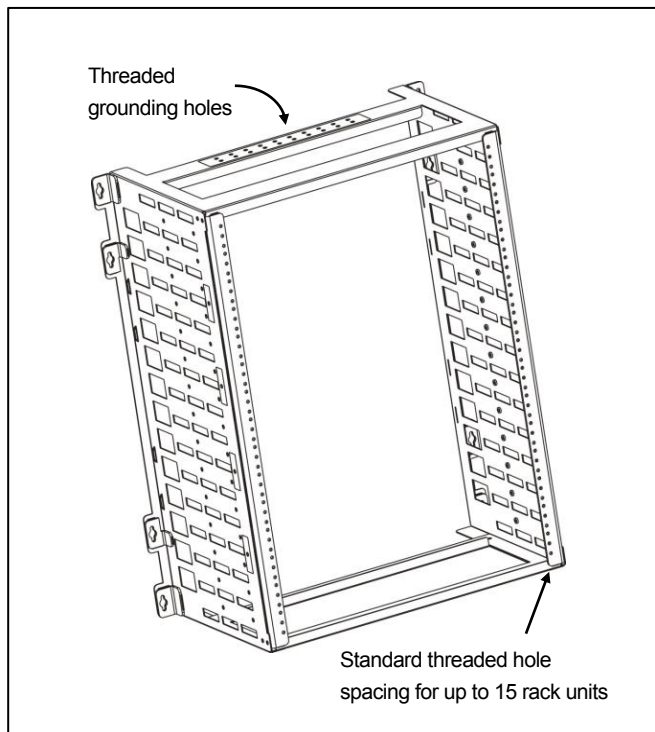
Figure 3. WR-15U Features
