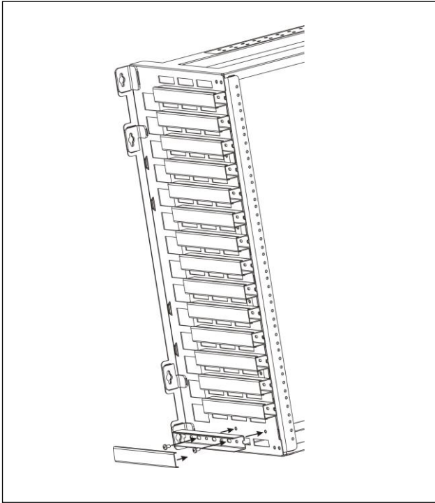
Figure 8. Cable guide installation
